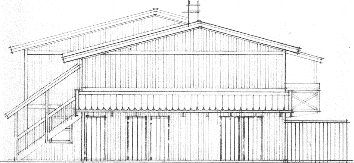
GAVELFASAD
